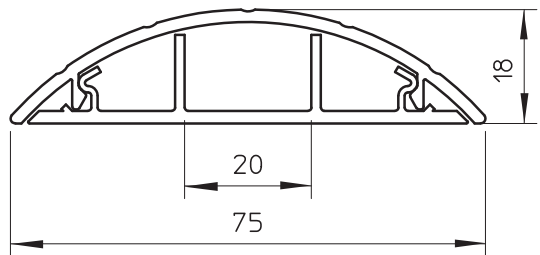
Trunking cover and base with base perforation.
